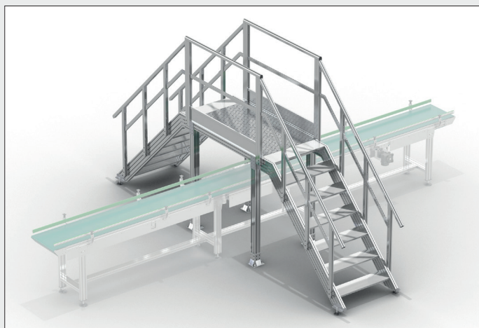
PASSERELLE SCAVALCAMENTO LINEA WALKWAYS TO OVERTAKE THE LINE
